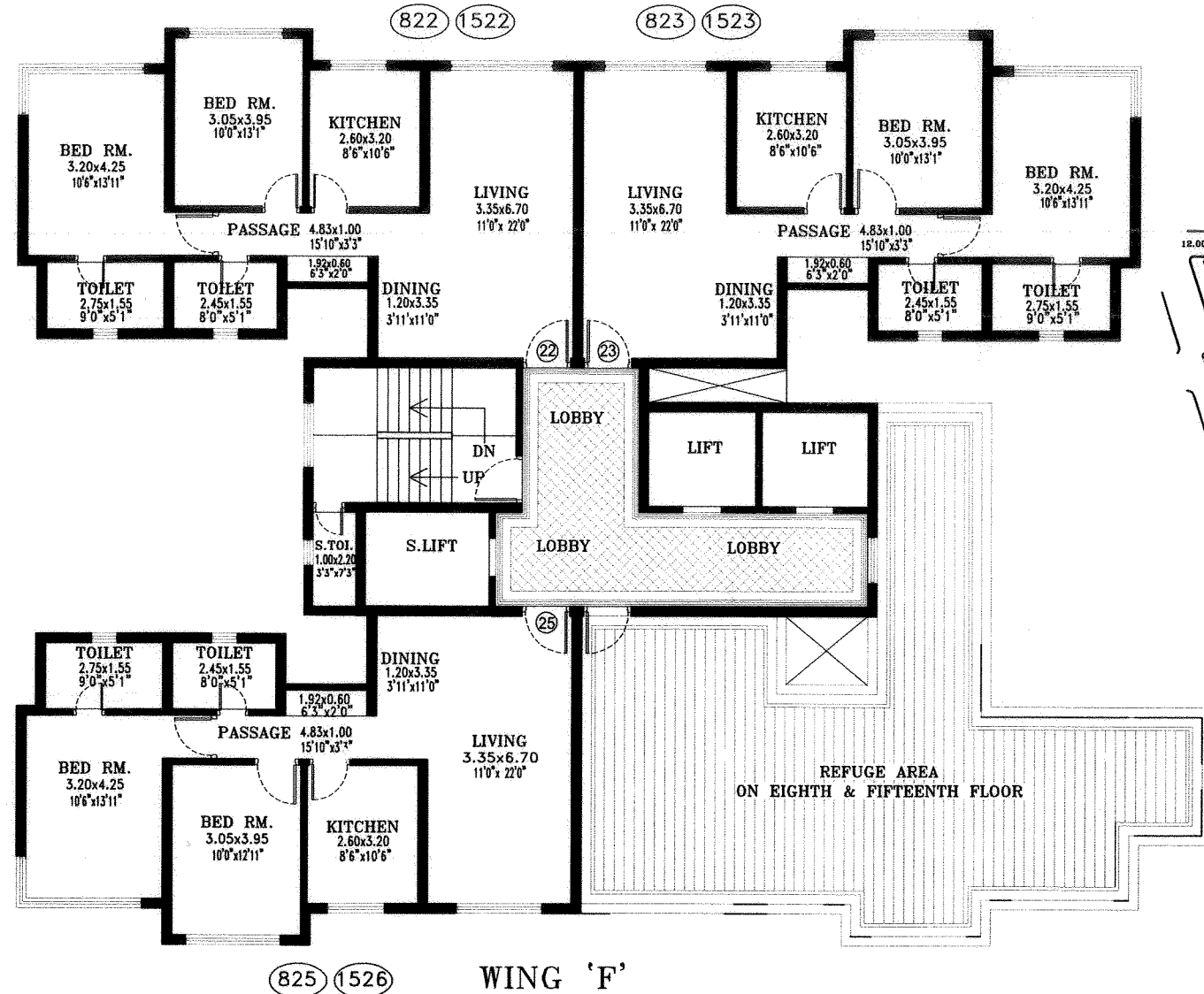
TENTATIVE EIGHTH & FIFTEENTH FLOOR PLAN
